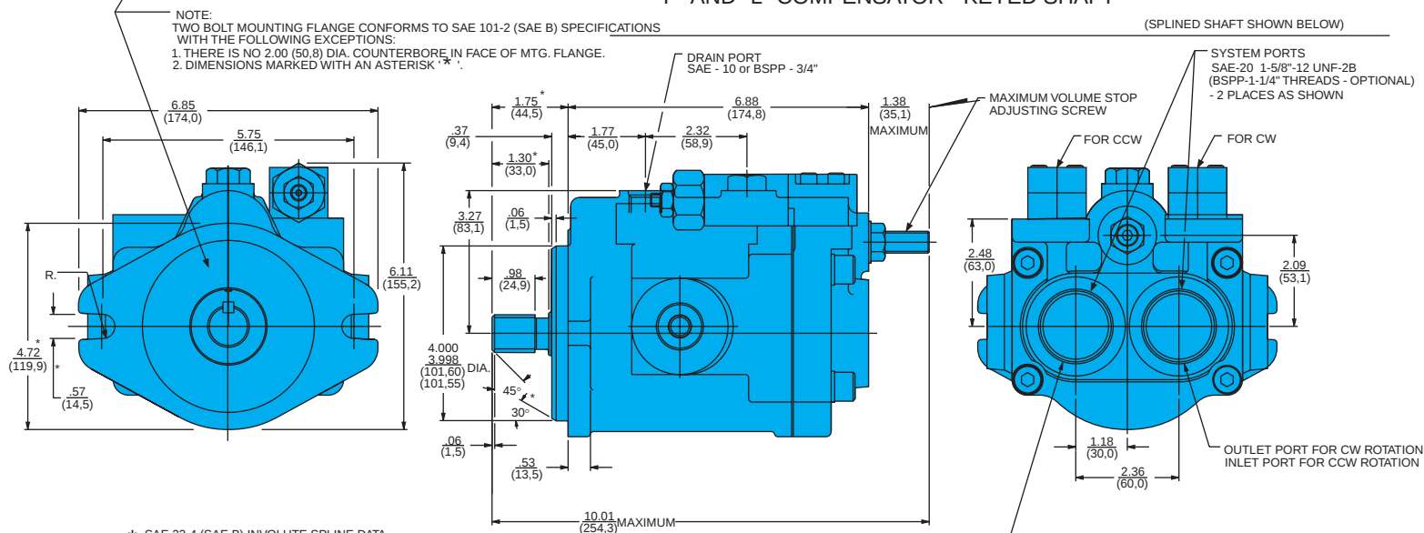
"F" AND "L" COMPENSATOR - KEYED SHAFT
