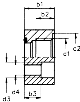
with G-thread
