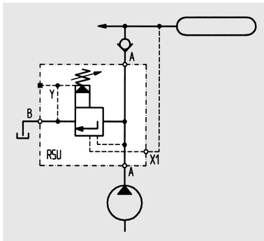
Accumulator system with Unloading Valve R5U
