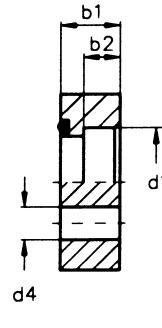
socket weld
